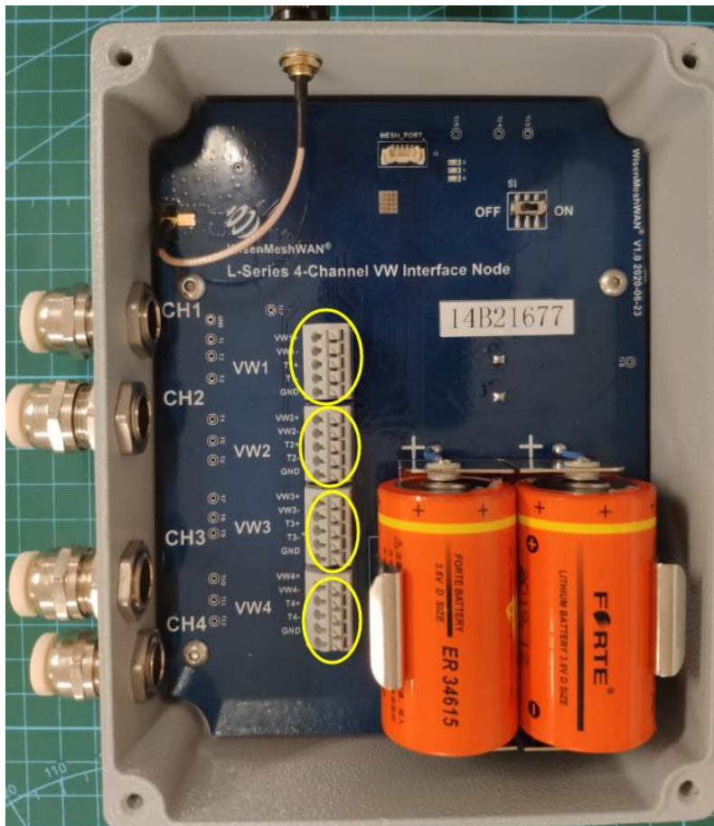
Figure 4. VW Sensor Connections (VW+, VW-, T+, T-, GND).
